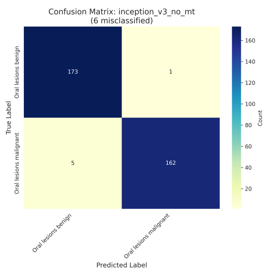
(j) Inception-V3 (No MT)
