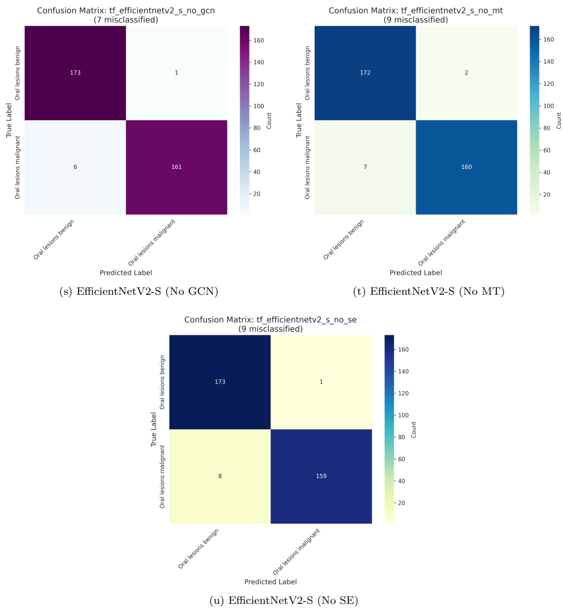
Supplementary Fig. S4. Confusion matrices related to oral dataset with respect to different models
